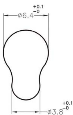
MOUNTING HOLE
