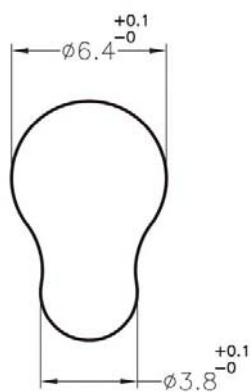
MOUNTING HOLE
