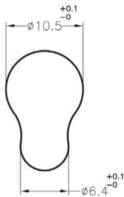
MOUNTING HOLE
